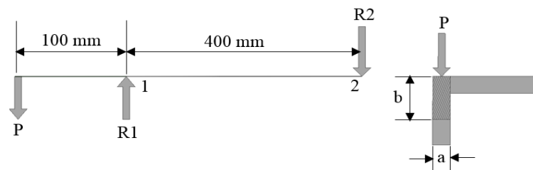
Figure 10. Free body diagram of part C
