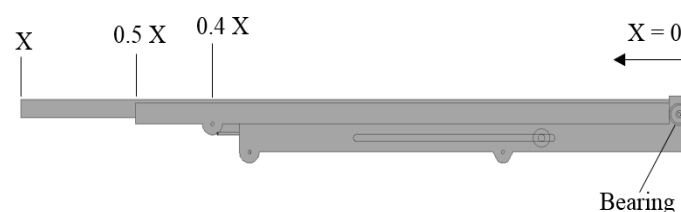
Figure 6. The side view proposed solar photovoltaic tilting platform at an angle \theta = 0^\circ
