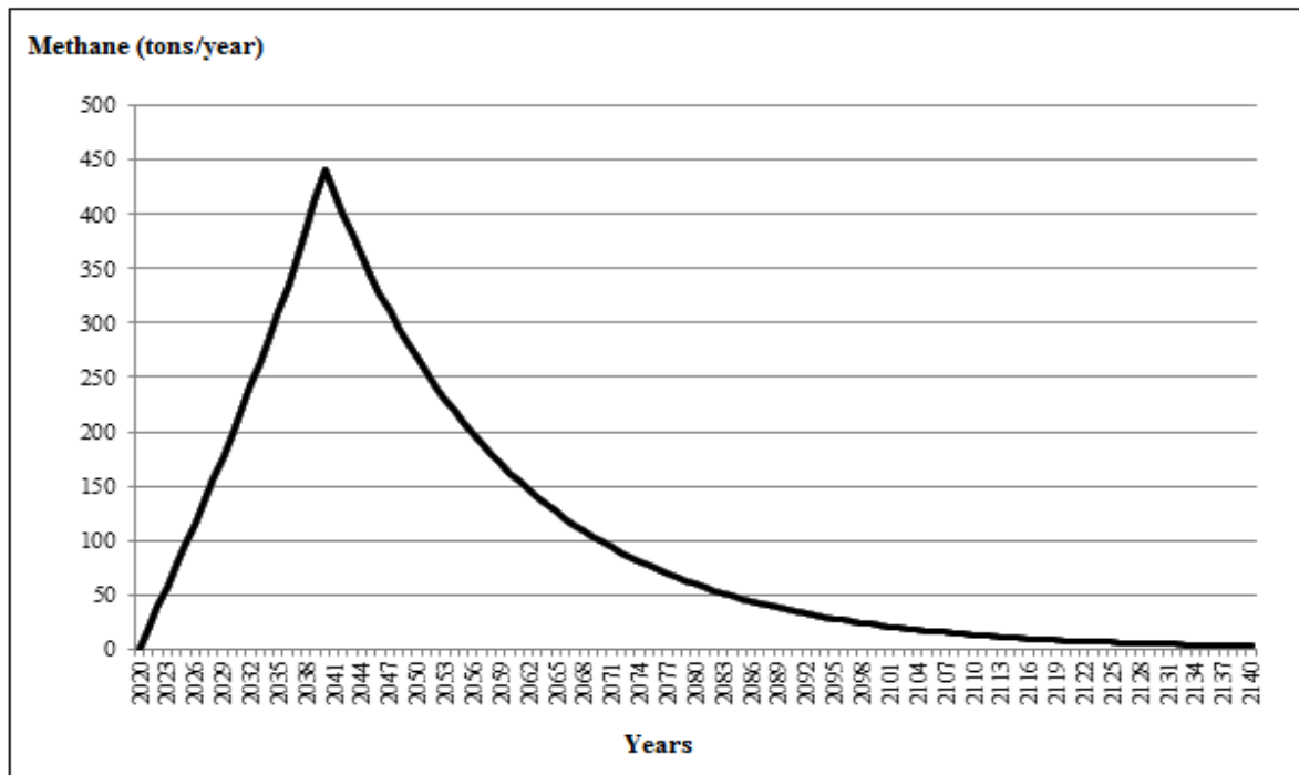
Figure 2. The methane production profile of the Edirne Solid Waste Landfill Facility
