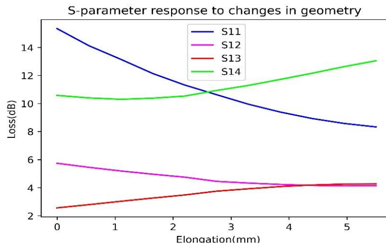
Figure 3. S parameter response to changes in geometry
