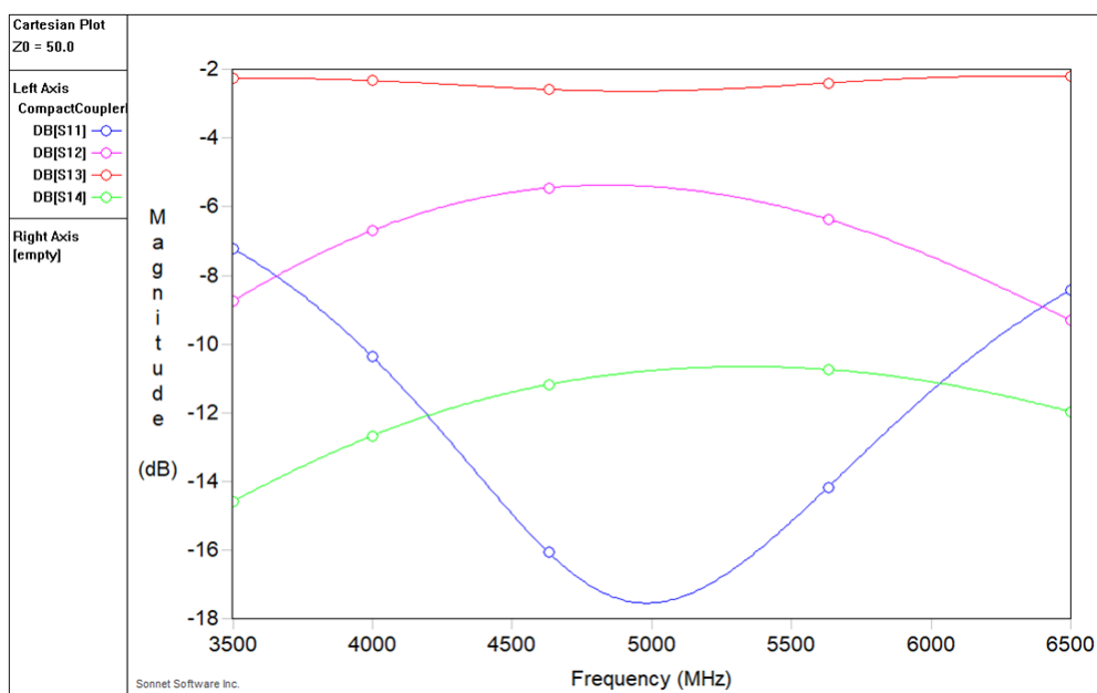
Figure 2. S-parameters
