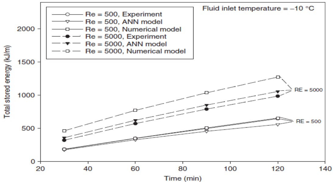
Figure 7. Variation of total stored thermal energy with time, using the ANN approach, the numerical model, and experimental data, for Re = 500 and 5000 and a HTF inlet temperature of -10\text{ }^{\circ}\text{C} [35]
