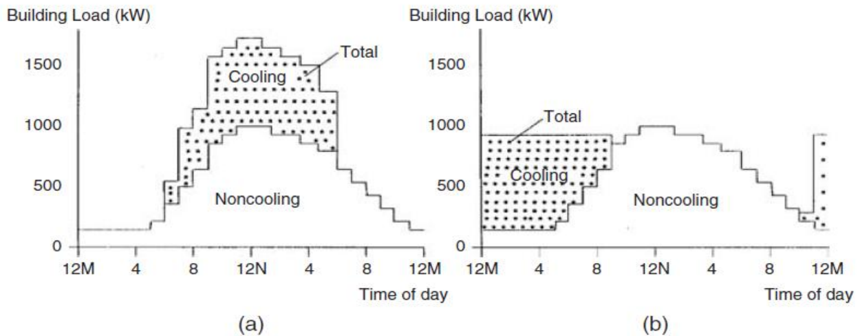
Figure 2. Daily load profiles of a building energy load: (a) no storage and (b) full storage [18]
