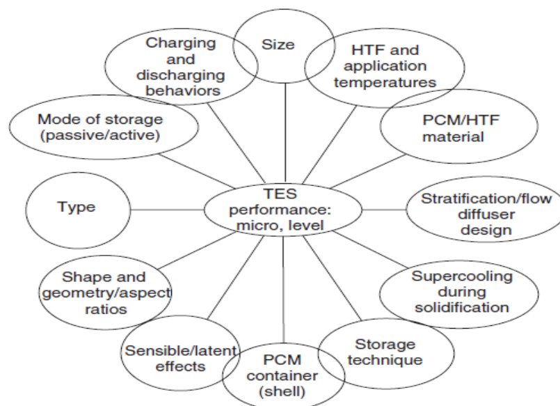
Figure 5. Parameters that affect TES performance at the micro level [13]
