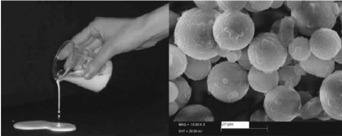
Figure 6. Flowing microencapsulated PCM as a phase-change slurry [29]
