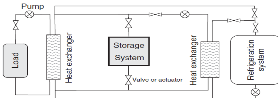
Figure 3. A cooling load serviced by a refrigeration system that incorporates thermal storage
