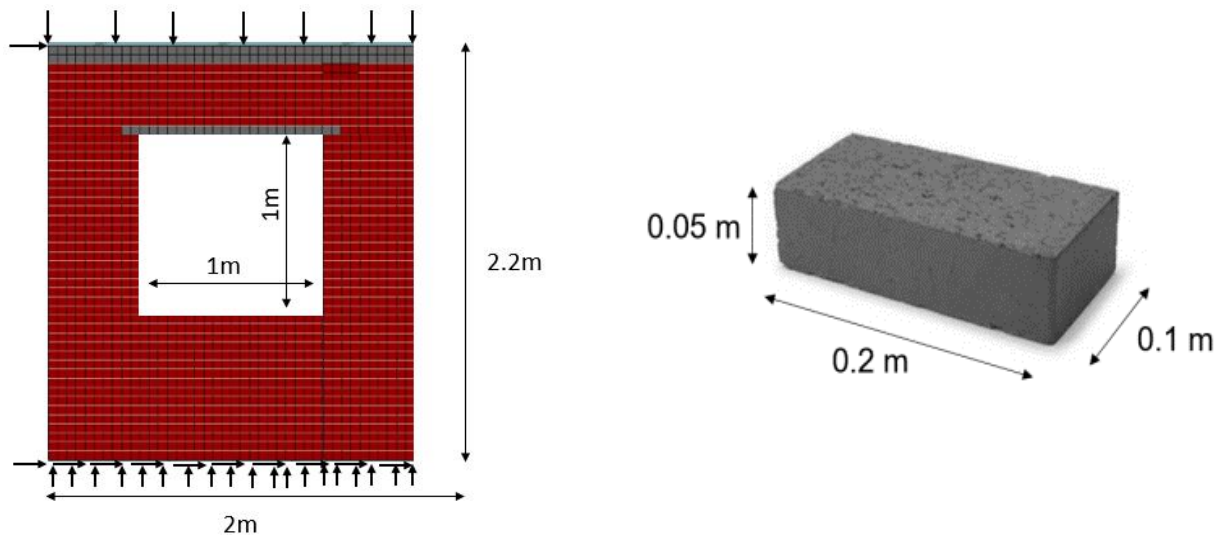
Figure 2. Description of the masonry wall with boundary condition and mesh size of 0.05mm; Details of the brick used in the current study
