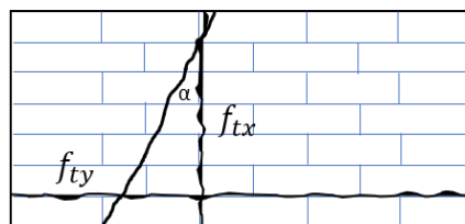
Figure 1. General characteristic of the Engineering Masonry model
