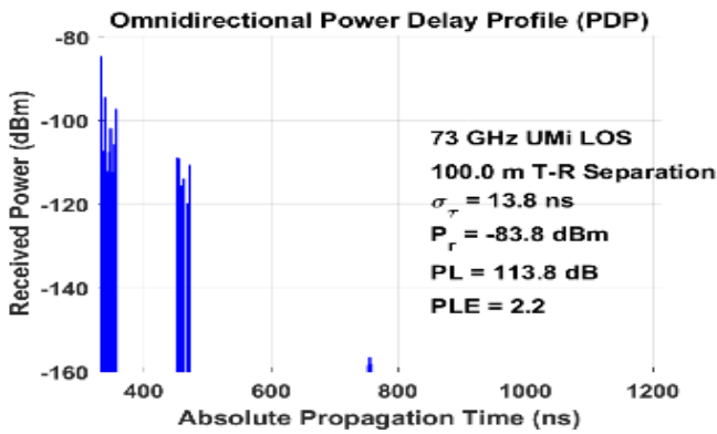
(e) The Co-Pol for 73 GHz
