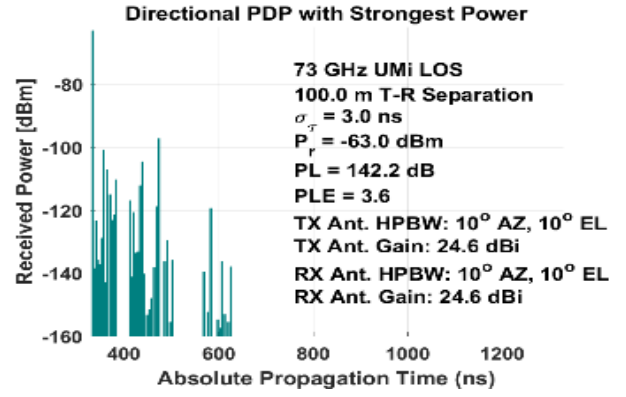
(f) The X-Pol for 73 GHz
