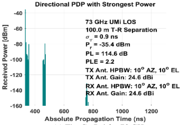
(e) The Co-Pol for 73 GHz
